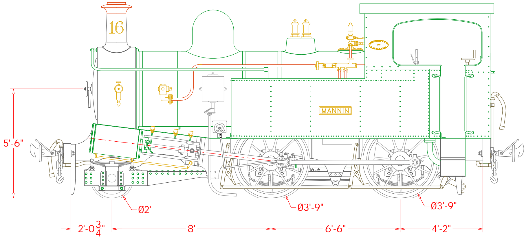
Beyer Peacock 2-4-0 Side Tank (Order No 144) Beyer Peacock Progress No. 6296 Isle of Man Railway 1926
