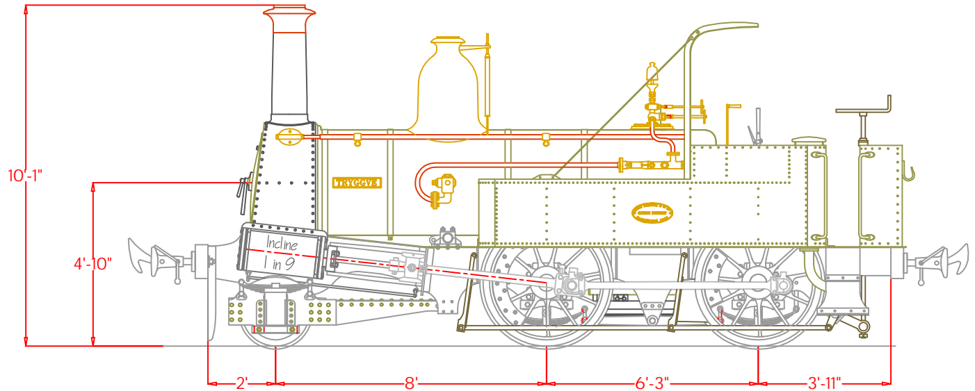
Beyer, Peacock & Co., Order No. 2000 of 1866 - Two 3' 6" Gauge 2-4-0t Locomotives for the Norwegian Government
