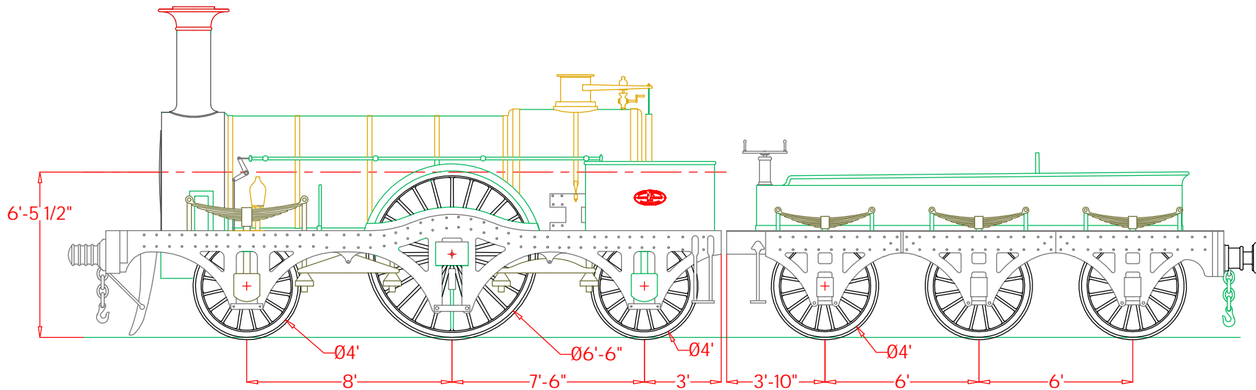
Beyer, Peacock & Co. Order Number 5 Beyer Peacock Progress Numbers 1 to 4 and 15 to 18 Seven 2-2-2 Standard Gauge Locomotives for the Great Western Railways. (Progress No. 1 to 4, 15 to 18)
