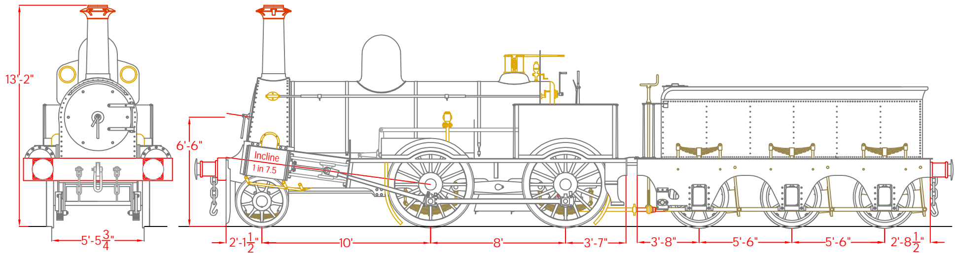
Beyer, Peacock & Co., Order No. 621 of 1862 - 41 5' 5 3/4" Gauge 2-4-0 Tender Locomotives for the Tudela & Bilbao Railway.
