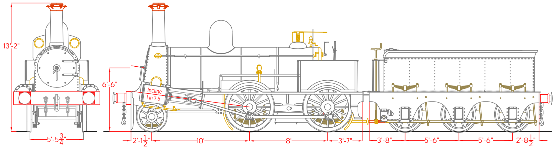
Beyer, Peacock & Co., Order No. 621 of 1862 - 41 5' 5 \frac{3}{4} " Gauge 2-4-0 Tender Locomotives for the Tudela & Bilbao Railway.
